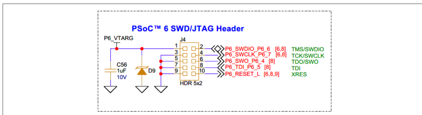
Figure 25 PSOC™ 6 SWD/JTAG header interface schematic
