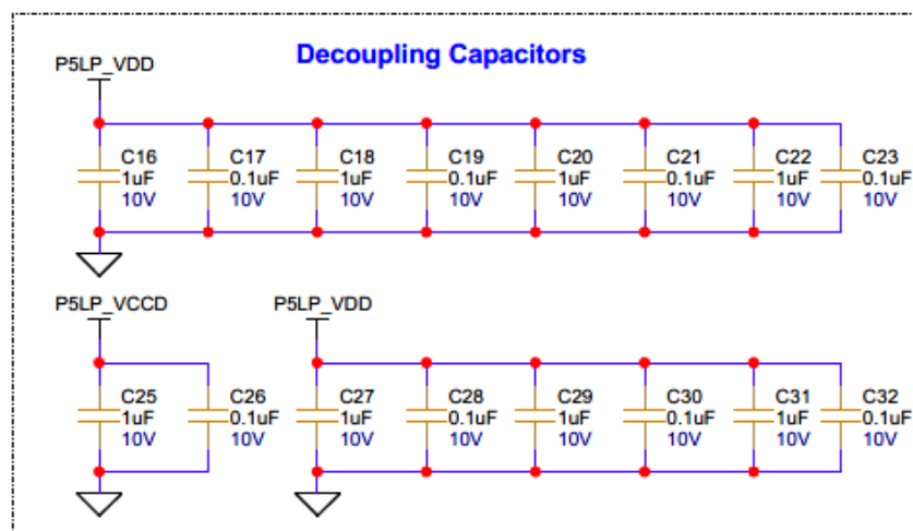
Figure 18 Schematic of PSOC™ 5LP based KitProg3
