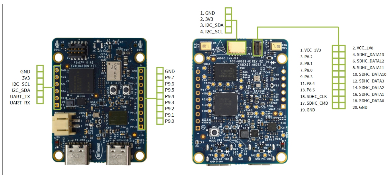
Figure 2 Board pinout
